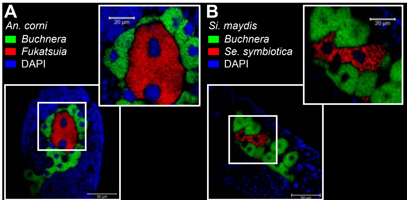
Figure 6. Location and morphology of co-obligate symbionts in selected aphid species. Merged FISH microscopic images of aphid embryos from (A) An. corni (lateral) (B) Si. maydis (tilted lateral). Co-obligate symbionts' signal is shown in red, Buchnera 's in green, and DAPI's (staining DNA, highlighting host nuclei) in blue. Thick white boxes indicate the magnified region depicted in the top-right of each panel. The scientific name for each species along with the false colour code for each fluorescent probe and its target taxon are shown at the top-left of each panel. Unmerged images can be found in https://doi.org/10.5281/zenodo.6394197 .
