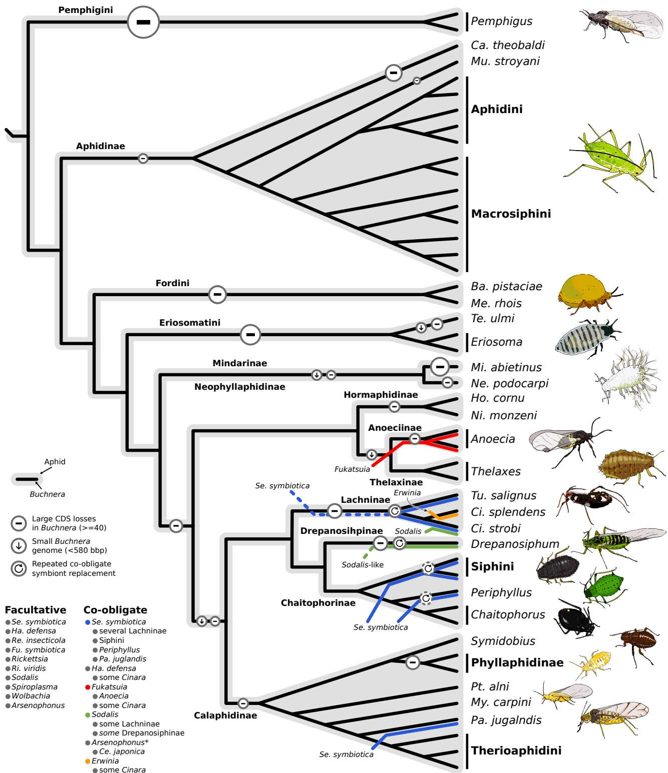
Figure 7. Evolutionary history of co-obligate symbioses in Aphididae. Diagram summarising results obtained from the genomic analysis presented in this work. Cladogram was made using the reconstructed phylogeny for Buchnera symbionts. Black lines in the cladogram represent Buchnera . Coloured lines are used to represent the acquisition of co-obligate symbionts. Dotted lines represent uncertainty in the acquisition of a specific taxa. Dotted circles represent uncertainty in symbiont replacement dynamics within the aphid lineage. On the right, aphid cartoons depicting variety of species across the Aphididae.
