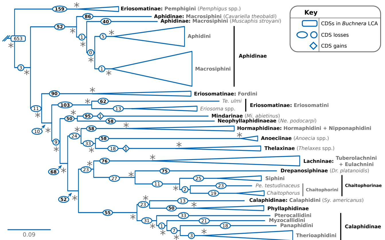
Figure 2. Phylogenetic relationships of Buchnera . Truncated Bayesian phylogenetic tree based on concatenated single-copy core proteins of selected Buchnera . Branches were collapsed on the basis of their aphid hosts' subfamily classification. At the right of leaves and clades, names of aphid subfamilies and tribes are shown in bold in black and grey colours, respectively. When a subfamily is only represented by the Buchnera strain of one aphid species or genus, it is indicated in between parentheses. Given that fliM+fliN and fliO+fliP often occurred as fused genes, they were each counted as one protein cluster instead of two. An asterisk at nodes stands for a posterior probability of 1. Escherichia coli , Pantoea ananatis , and Erwinia spp. were used as outgroups. Full phylogenetic tree can be found at (supplementary figure S1, Supplementary Material online).
