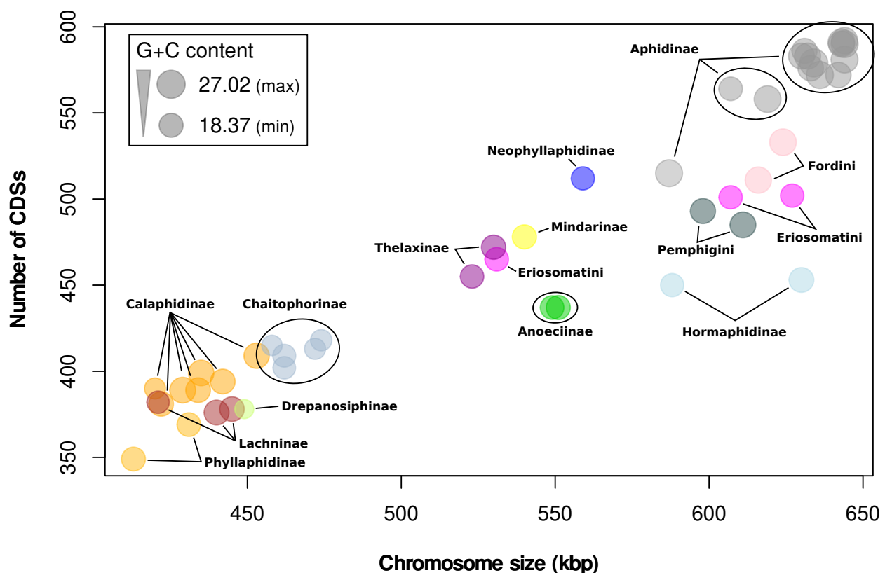
Figure 1. Relationship of genome size vs. CDS content in Buchnera genomes. Scatter plot illustrating the diversity of genome size, number of CDSs and G+C content of selected Buchnera genomes. Taxonomic classification of aphid host is displayed in bold black lettering. Dots are colour coded according to the host's subfamily or tribal classification. Size of circles represent the G+C content as shown in the legend box scale key.
