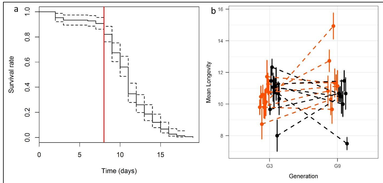
262 263 Figure 2. Evolution of fly survival. (a) Survival of female flies in the water condition at G3. Dotted lines represent the 264 95 % confidence interval. The red vertical line shows the age (8 days) at which reproduction was enforced during the 265 experimental evolution. The corresponding figure for the paraquat condition is provided as supplementary material (b) 266 Mean longevity ( \pm standard error) in all lines in the paraquat (orange) and water (black) conditions, at generations 3 267 and 9.
