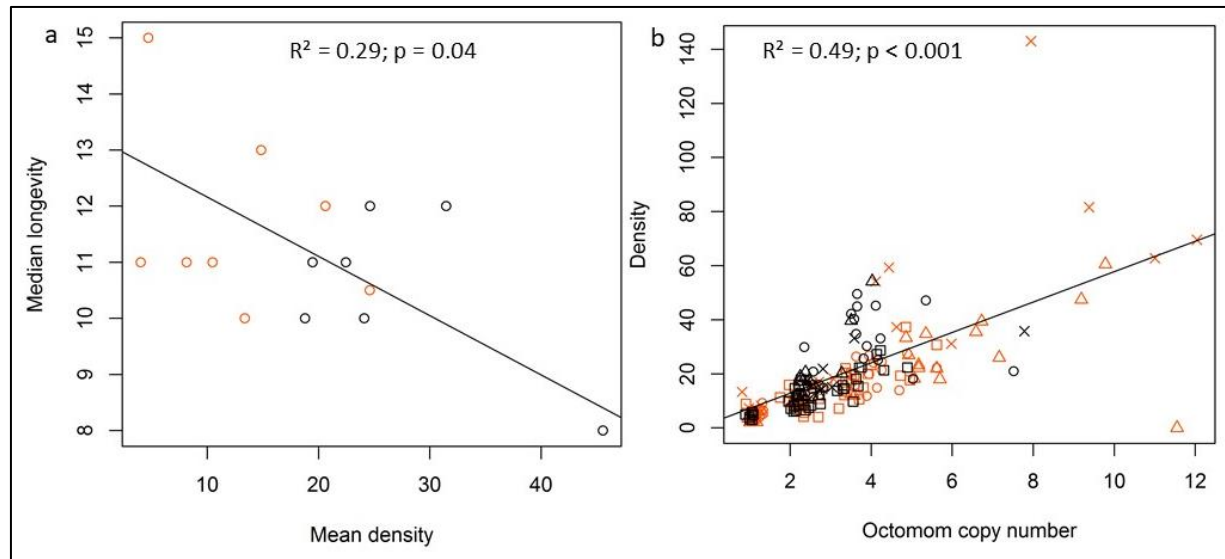
318 319 Figure 4. (a) Correlation between Wolbachia density and fly survival. Each circle represents a line in the paraquat 320 (orange) or water (black) condition, at G9. The black line represents the regression of median longevity on mean 321 density (data for both conditions are pooled, as the treatment effect was found not to be statistically significant). 322 Statistics from Pearson's correlation test are indicated. (b) Correlation between Wolbachia density and octomom copy 323 number. Each symbol represents an individual fly, from the paraquat (orange) or water (black) condition, at G2 324 (squares), G9 (circles), G12 (triangles), or G17 (crosses). The black line represents the regression of density on 325 octomom copy number. Statistics from Pearson's correlation test, with all conditions pooled together, are indicated.
