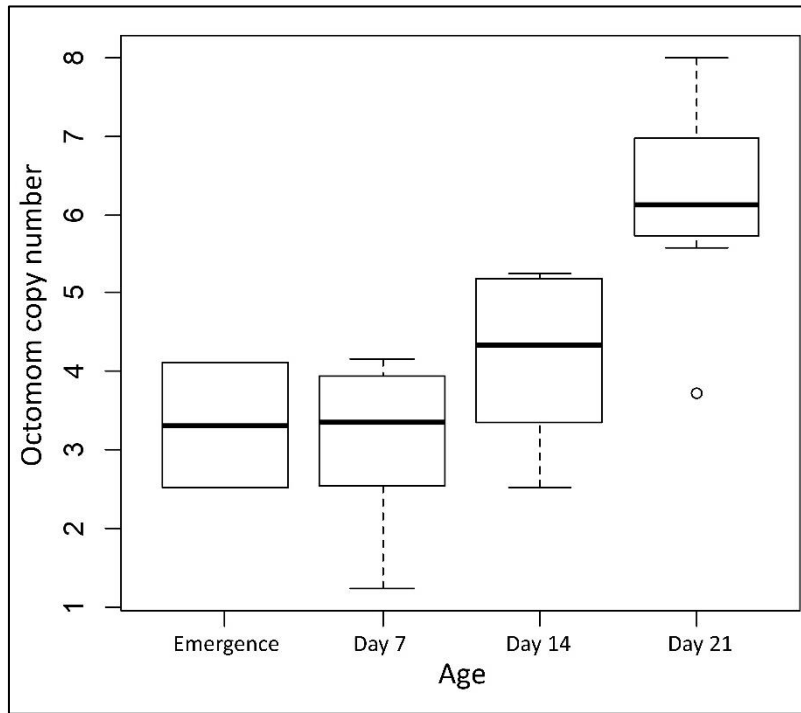
363 364 Figure 5. Relationship between the age of the fly and the octomom copy number of wMelPop . Data pooled from two 365 treatments (paraquat and water), as neither the interaction between age and treatment ( F_{1,22}=2.79 , p=0.11 ) nor the 366 treatment effect ( F_{1,23}=0.14 , p=0.72 ) were significant.
