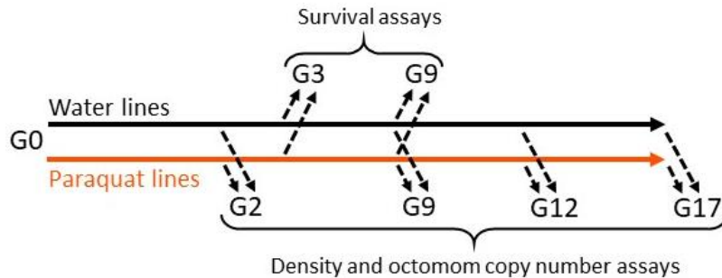
137 138 Figure 1. Summary diagram of the experimental evolution experiment, showing the generations (G0-G17) at which 139 the different measurements were performed.
