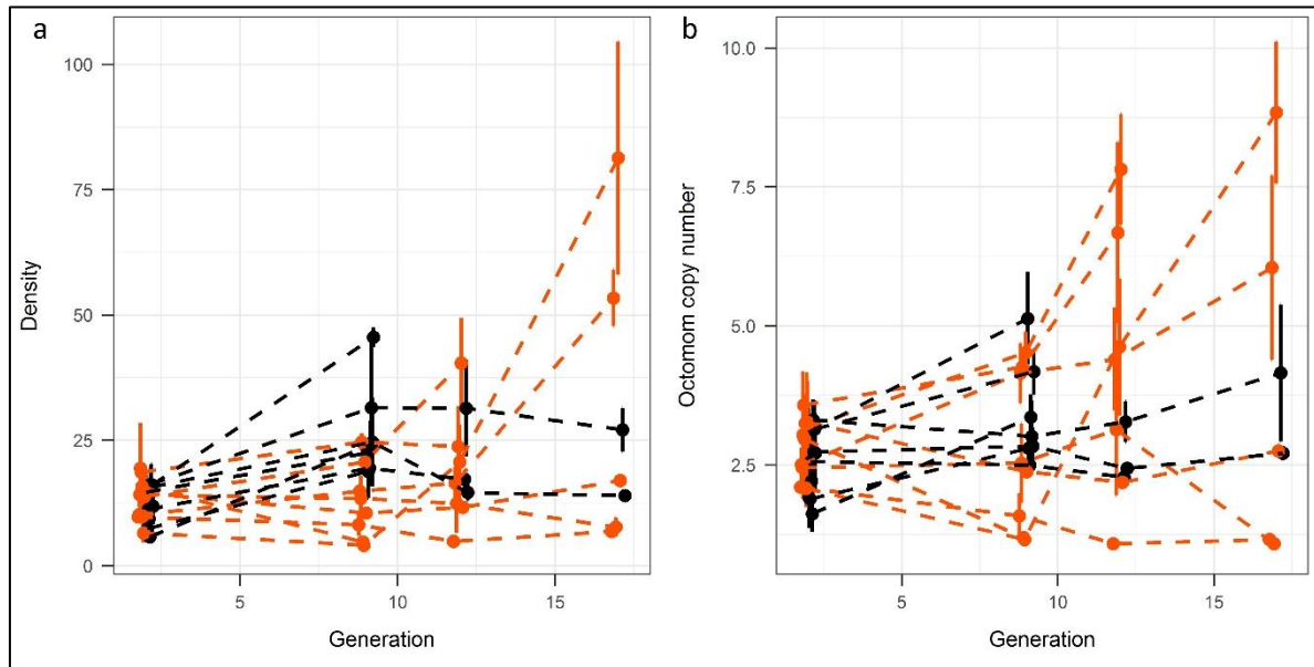
282 283 Figure 3. Evolution of Wolbachia density and octomom copy number. (a) Mean Wolbachia relative density ( \pm standard 284 error) in all lines in the paraquat (orange) and water (black) conditions, at generations 2, 9, 12 and 17. (b) Mean 285 octomom copy number ( \pm standard error) in all lines in the paraquat (orange) and control (black) conditions, at 286 generations 2, 9, 12 and 17.
