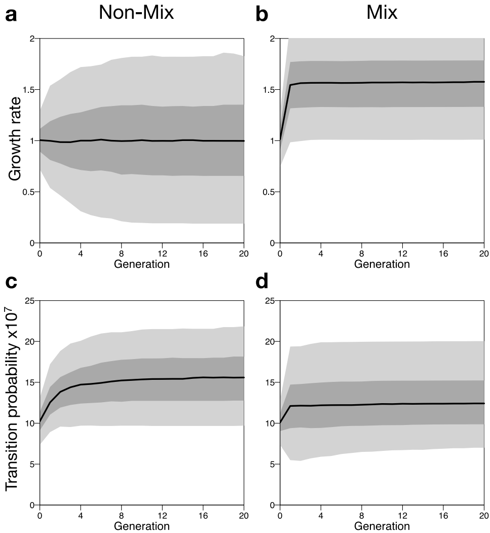
Supplementary Figure 1. Model dynamics with a random distribution of initial parameters (no tradeoff)
