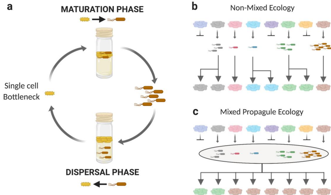
Figure 1. Experimental Regimes (a) A single ‘mat’ generation consists of a life cycle of two phases. The Maturation Phase is seeded with a single WS cell. SM cells arise within the mat and are harvested after six days of maturation by plating and collection of all SM colonies on agar plates. The SM propagule cells are transferred to a new microcosm to begin a three-day Dispersal Phase, during which WS mat-forming cells arise. At the end of the Dispersal Phase, cells from microcosms are plated once more, and a single WS colony (representative of the most common colony morphology type) is picked to seed the next generation. Mat extinctions occur if there are no SM cells after six days of the Maturation Phase, no WS cells after three days in the Dispersal Phase, or if the mat collapses during the Maturation Phase. (b) and (c) Schematic depiction of a population of eight genetically distinct groups (indicated by different colours) proceeding through one life cycle within their respective non-mixed (b) and mixed (c) ecologies.
