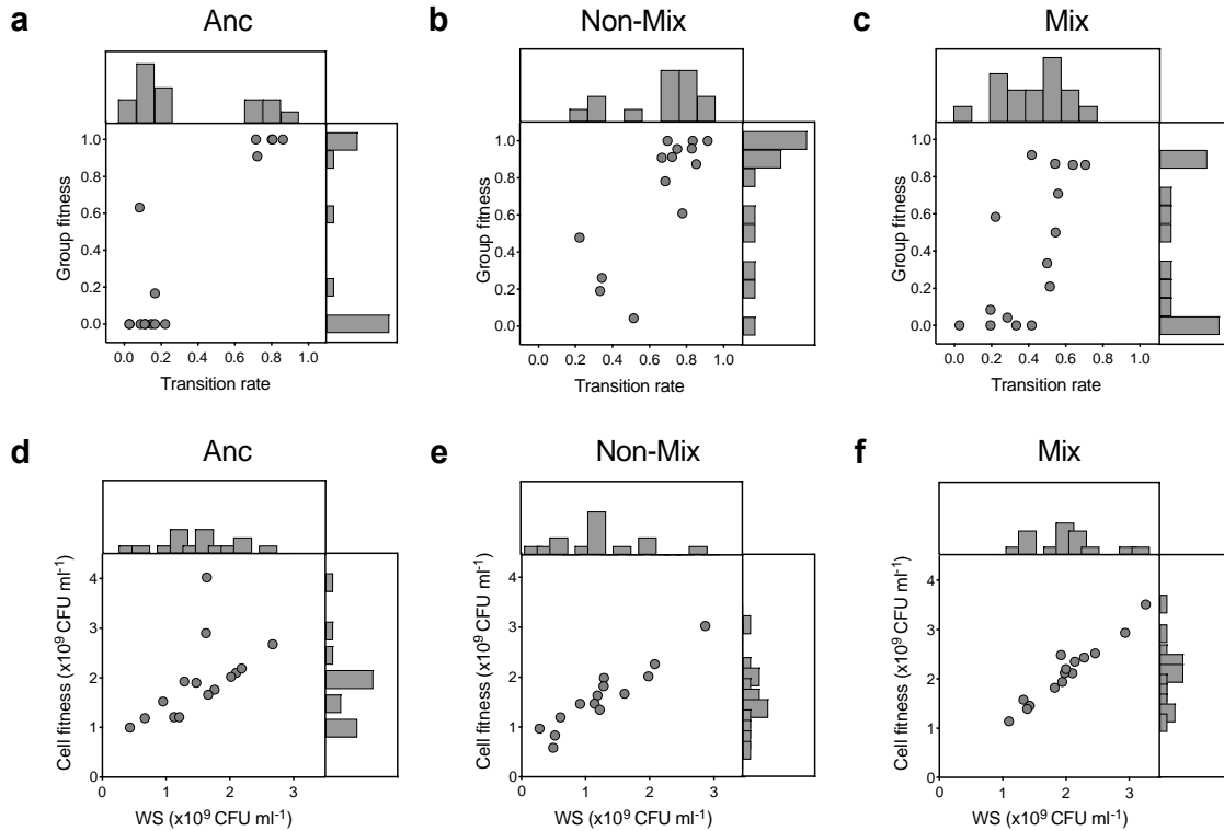
Figure 6. Relationship between life cycle traits and group and cell fitness. (a-c) Association of transition rate and group fitness in the ancestral populations (a), and in the Non-Mixed (b) and Mixed Propagule (c) Ecologies. (d-f) WS density is positively associated with cell fitness in the ancestral populations (d), and in the Non-Mixed (e) and Mixed (f) Propagule Ecologies. Group fitness is the proportion of derived offspring mats after one lifecycle relative to a genetically marked reference genotype. Dots represent the mean of eight lines per replicate population, which were assessed in three independent competition assays.
