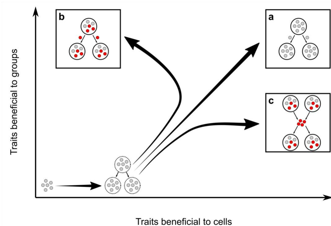
Figure 10. The origins of life cycles and the notion of fitness decoupling. Mode of group reproduction via a) fragmentation, b) a germ line (red) in a highly structured population and c) a germ line with propagule mixing, affects the emergence of individuality. Mode of group reproduction impacts the relationship between two levels of selection: the cell level (relative to the free-living state), and that of the emerging group. a) illustrates an example of a group that reproduces by fragmentation where fitness is ‘coupled’: group fitness is a by-product of the fitness of the constituent cells. Larger groups contain more cells and produce more offspring. This holds even when the reproductive life cycle involves a single-celled bottleneck – a feature that is expected to reduce within-group competition. b) and c) show examples of groups that reproduce via a life cycle involving two cell types – one soma-like and the other germ-like. Such two-phase life cycles allow possibility for traits determining a necessary developmental programme to evolve independent of the growth rate of cells that comprise the nascent organism. This paves the way for the emergence of new kinds of biological individual where group fitness ‘decouples’ from cell fitness.
