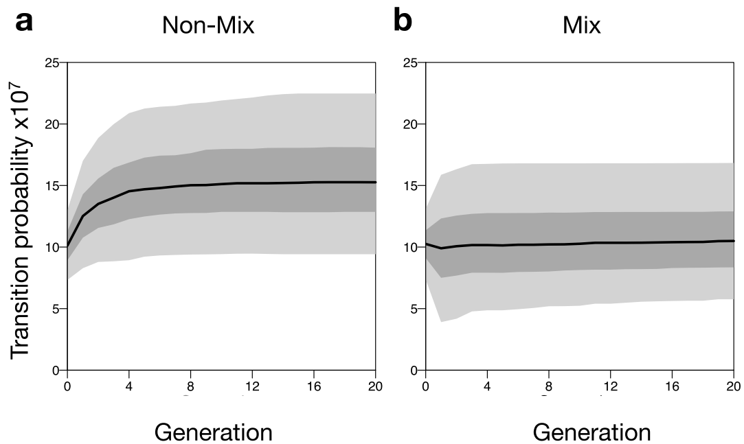
Figure 8 Simulated dynamics of the average transition probability in (a) the Non-Mixed Ecology, and (b) the Mixed Propagule Ecology. Black lines represent median transition rate values across 600 independent realizations of the respective selection regime. Dark grey areas indicate a 50% confidence interval, while light grey areas indicate a 95% confidence interval.
