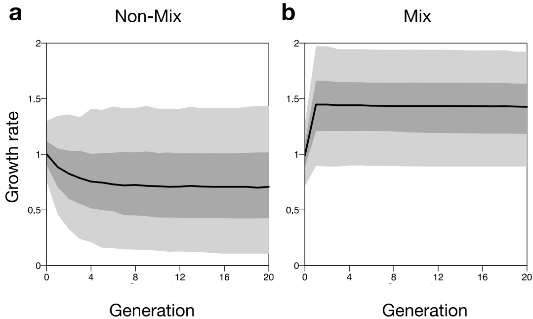
Figure 7. Simulated dynamics of the average cell growth rate in (a) the Non-Mixed Ecology, and (b) the Mixed Propagule Ecology. Black lines represent median growth rate values across 600 independent realizations of the respective selection regimes. Dark grey areas indicate a 50% confidence interval, while light grey areas indicate a 95% confidence interval.
