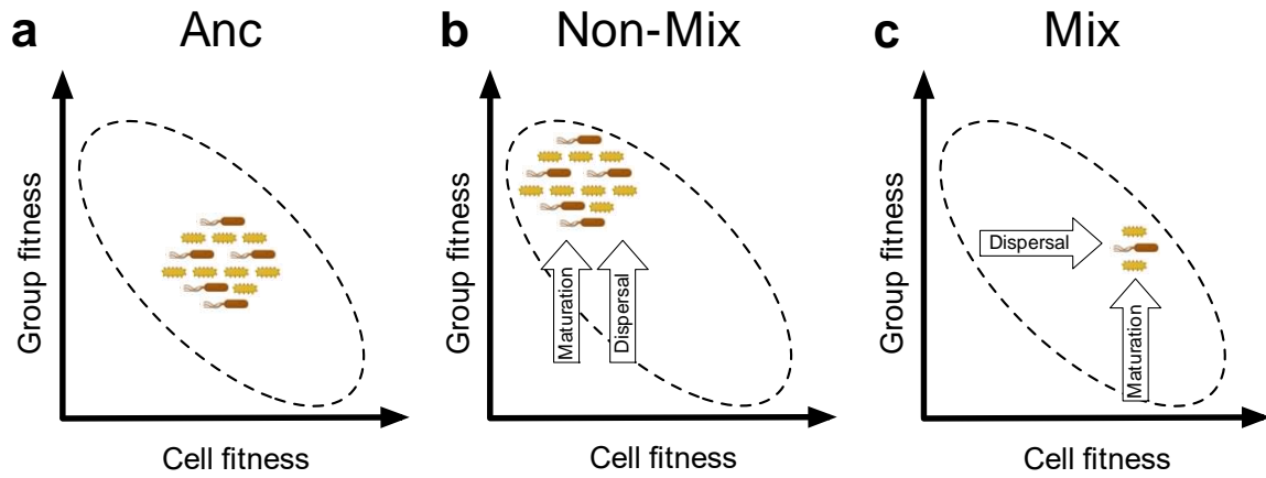
Figure 9. Ecological conditions can steer the evolution of traits in opposite directions. A meta-population is depicted by the cloud of cells, where the position of the cloud represents the average fitnesses and the size of the cloud represents the diversity within a meta-population. The group and cell fitness are subjected to a tradeoff (dashed line eclipses) and cannot be optimized simultaneously. Arrows indicate the direction of selection applied by Maturation and Dispersal Phases of the life cycle. Both phases selected for increased transition rate in the Non-Mixed Ecology, whereas in the Mixed Propagule Ecology the Dispersal Phase promoted increased cell numbers at the expense of transition rate. The mixing procedure resulted in significantly decreased diversity, which further limited opportunity for adaptive evolution of groups.
